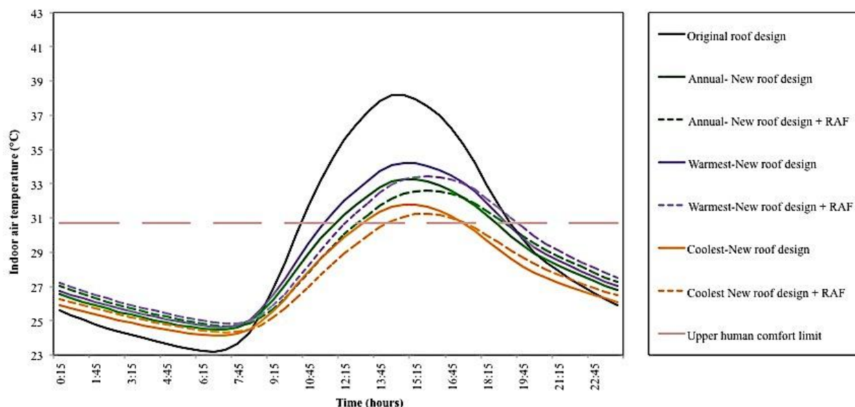
Fig. 3. Daily average indoor air temperature of the freshwater prawn hatchery building during the warmest month, coolest month and annual overall.
