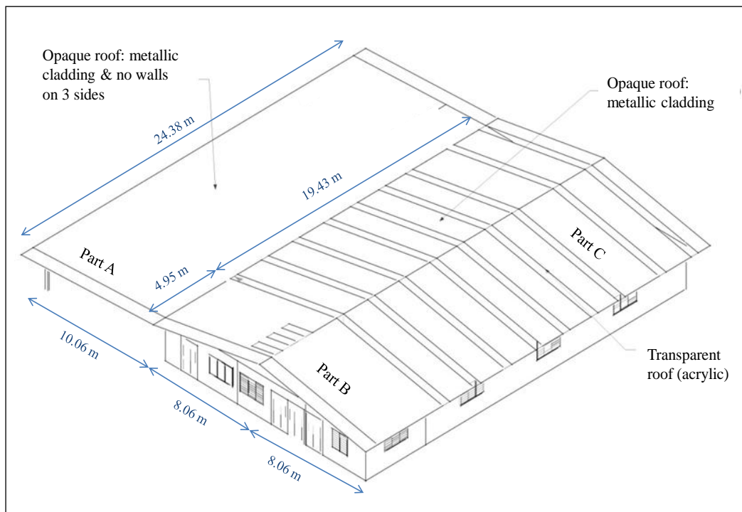
Fig. 1. Original roof design of the freshwater prawn hatchery building showing measurements of the plan.
