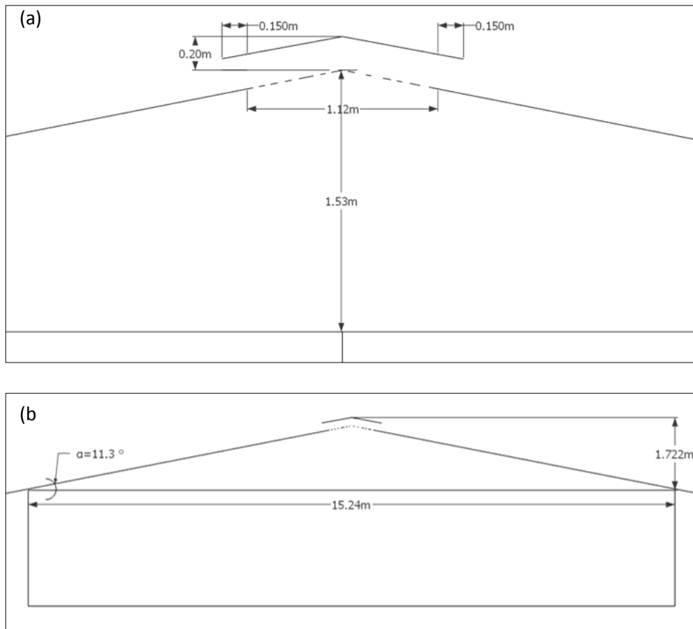
Fig. 2. The measurement of the monitor roof design of the freshwater prawn hatchery building. (a) small opening of the roof, (b) front view of the hatchery.
