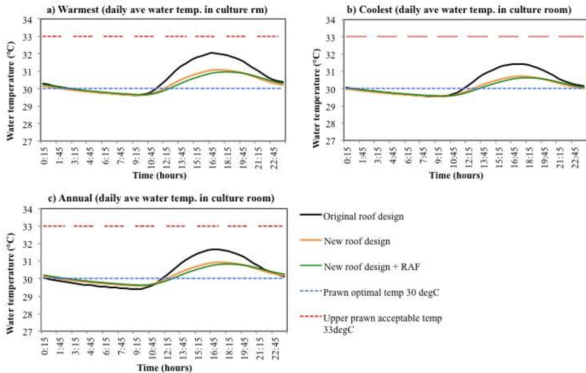
Fig. 5. Daily average water temperature in the culture room of the freshwater prawn hatchery building: (a) warmest month, (b) coolest month, (c) annual.
