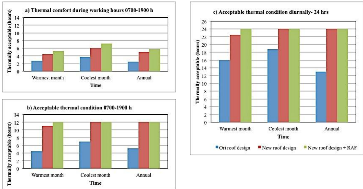
Fig. 4. Indoor thermal condition of the hatchery: (a) Working hours thermal comfort (0700 –1900 h), (b) Working hours acceptable thermal condition (0700-1900 h), (c) Acceptable thermal condition (diurnally - 24 h).
